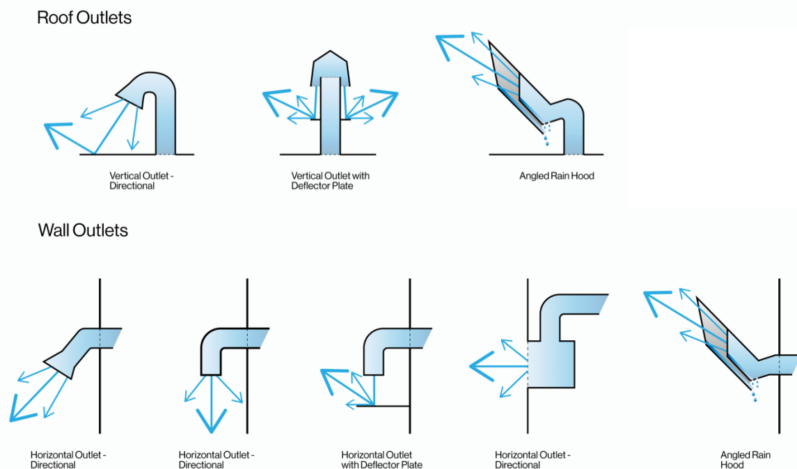
Figure 16. Examples of quench pipe outlet designs.
