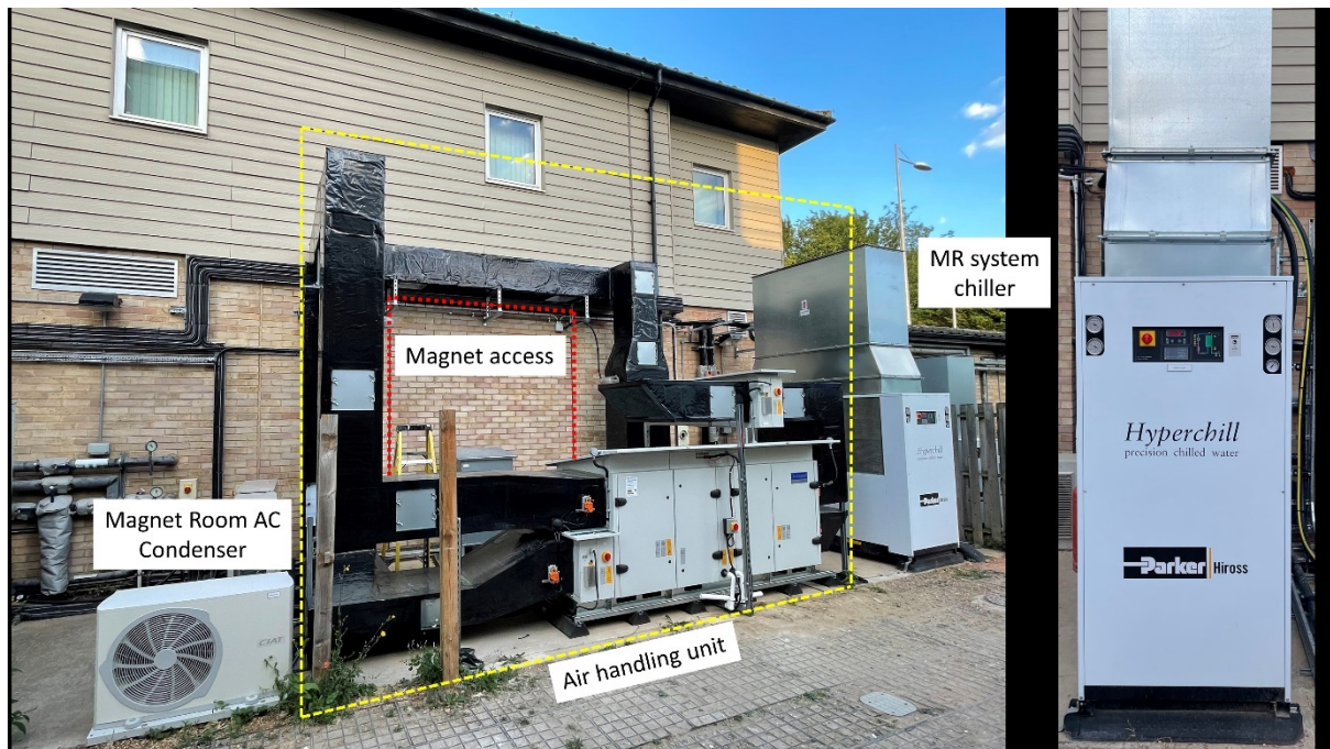
Figure 18. Example of MRI supporting plant. The air handling unit is highlighted by the yellow dotted box. Also shown is the condenser unit for the MR Examination room air conditioning and the MR chiller system that provides chilled water to the MR system heat exchanger located in the equipment room. The red dotted line partially shows the magnet access. This wall is demolished for installation/removal of the magnet.
